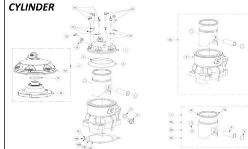
CILINDRO CYLINDER
