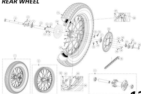
RUEDA TRASERA REAR WHEEL
