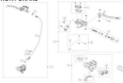
FRENO DELANTERO FRONT BRAKE
