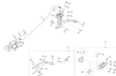
FRENO TRASERO REAR BRAKE
