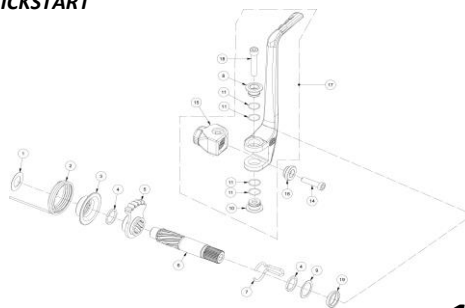
PEDAL DE ARRANQUE KICKSTART
