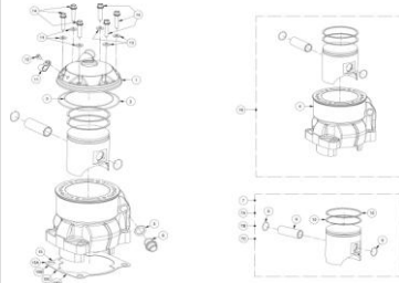
CILINDRO CYLINDER
