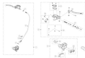
FRENO DELANTERO FRONT BRAKE
