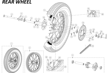
RUEDA TRASERA REAR WHEEL
