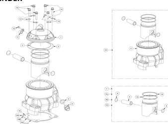
CILINDRO CYLINDER
