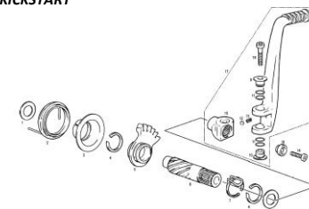
PEDAL DE ARRANQUE KICKSTART
