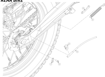
TREN TRASERO REAR BIKE
