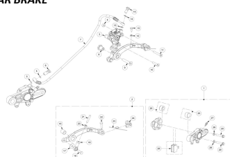
FRENO TRASERO REAR BRAKE
