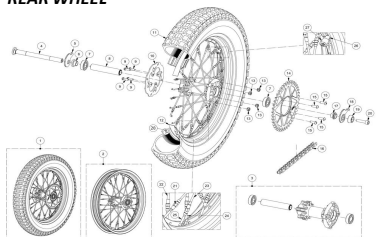
RUEDA TRASERA REAR WHEEL
