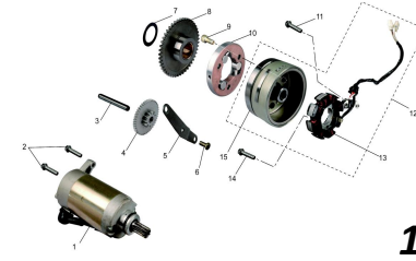
MOTOR DE ARRANQUE / ENCENDIDO ELECTRIC STARTING MECHANISM / GENERATOR
