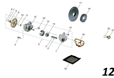
BOMBA ACEITE OIL PUMP
