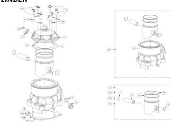
CILINDRO CYLINDER
