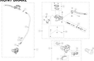
FRENO DELANTERO FRONT BRAKE
