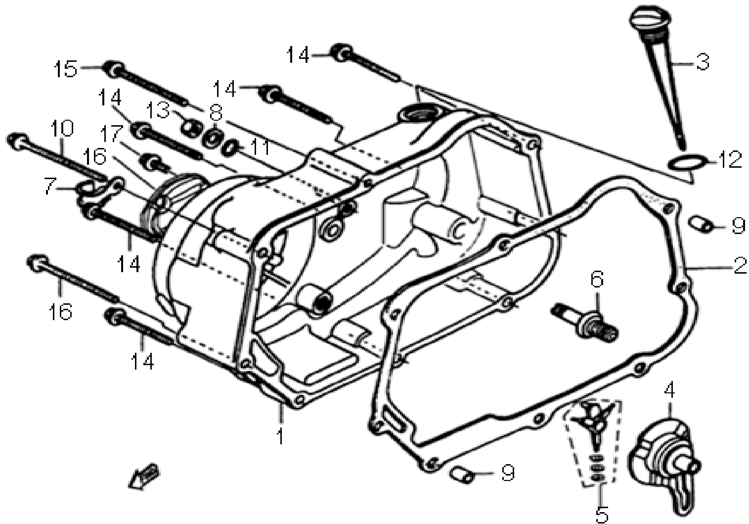
FIG. 4 RIGHT CRANKCASE COVER
