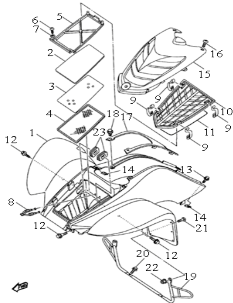
FIG. 20 FRONT FENDER
