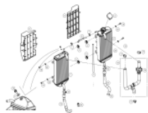
Radiator
