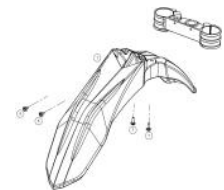
Front dender
