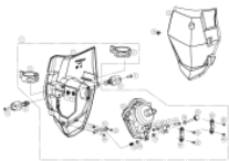
Head light
