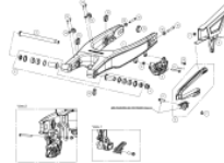
Swing Arm
