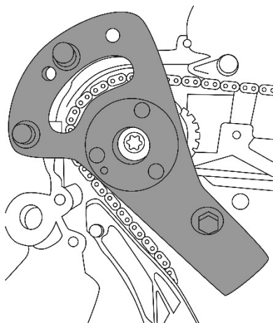
Exhaust Camshaft
