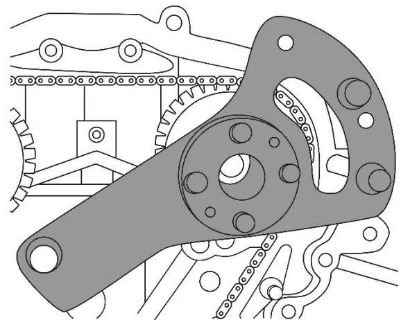
Inlet Camshaft
