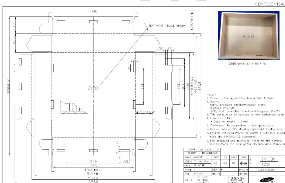
Fig. 2-2. Inner box package drawing.
